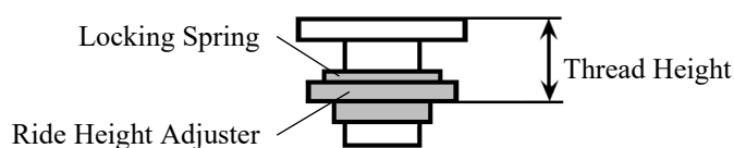
[Rear Ride Height Adjuster Assy]
